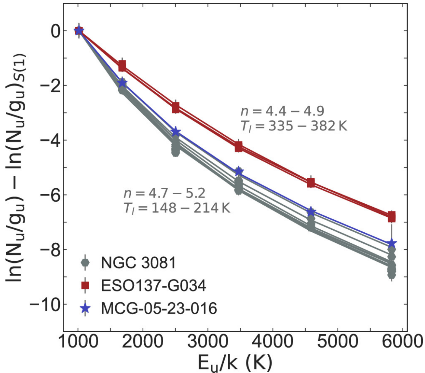
Figure 6. from Lulu Zhang et al 2024 Astrophys. J. Lett. 975 doi:10.3847/2041-8213/ad81d0 https://dx.doi.org/10.3847/2041-8213/ad81d0 © 2024. The Author(s). Published by the American Astronomical Society.
