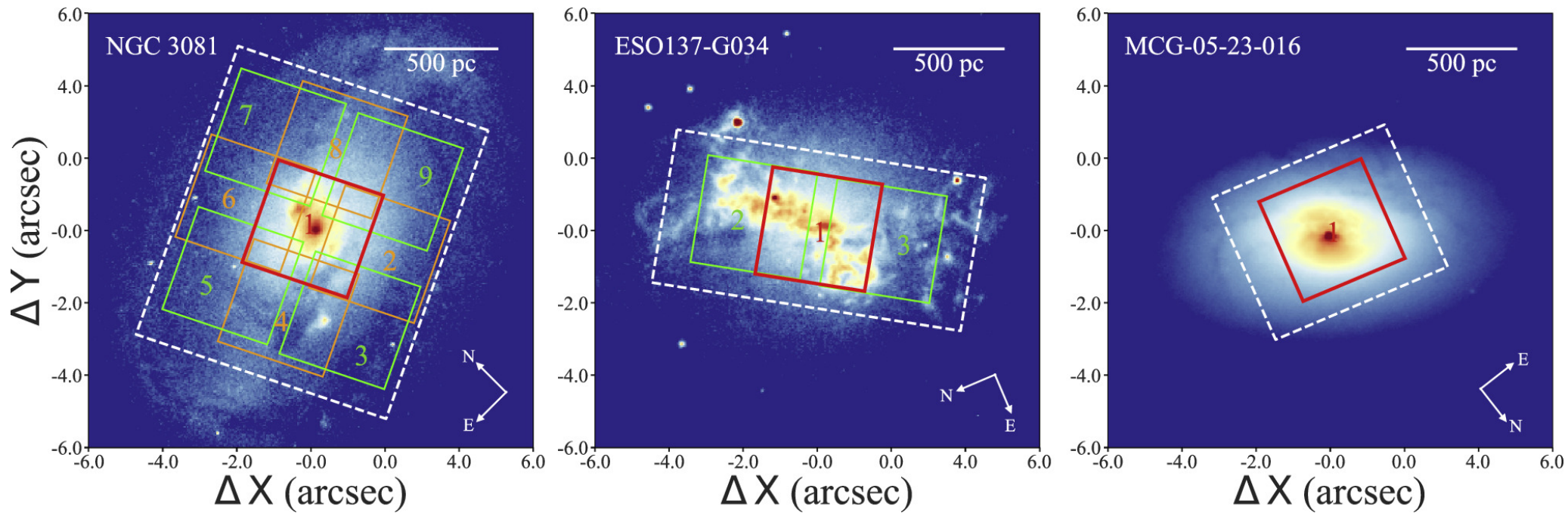
Figure 1. from Lulu Zhang et al 2024 Astrophys. J. Lett. 975 doi:10.3847/2041-8213/ad81d0 https://dx.doi.org/10.3847/2041-8213/ad81d0 © 2024. The Author(s). Published by the American Astronomical Society.
