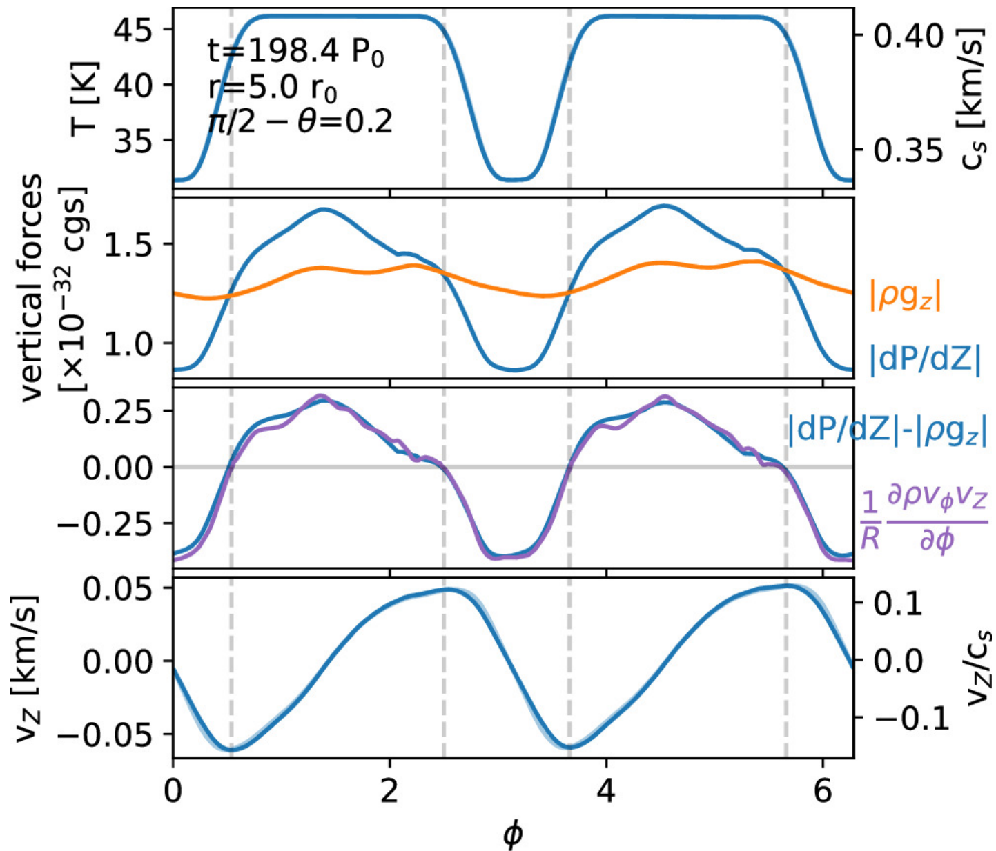
Figure 4. from Shangjia Zhang and Zhaohuan Zhu 2024 Astrophys. J. Lett. 974 doi:10.3847/2041-8213/ad815f https://dx.doi.org/10.3847/2041-8213/ad815f © 2024. The Author(s). Published by the American Astronomical Society.
