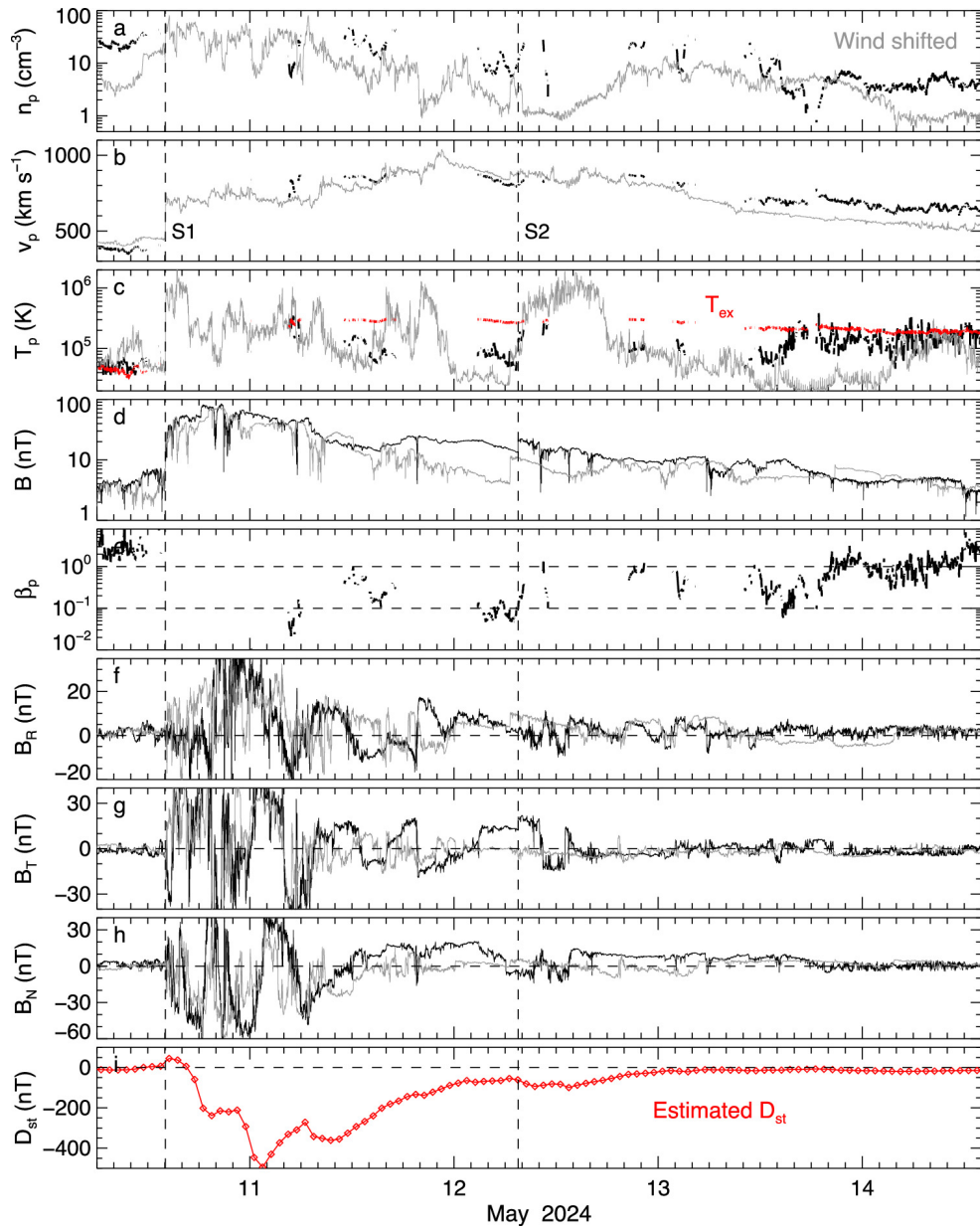
Figure 4. from Ying D. Liu et al 2024 Astrophys. J. Lett. 974 doi:10.3847/2041-8213/ad7ba4 https://dx.doi.org/10.3847/2041-8213/ad7ba4 © 2024. The Author(s). Published by the American Astronomical Society.
