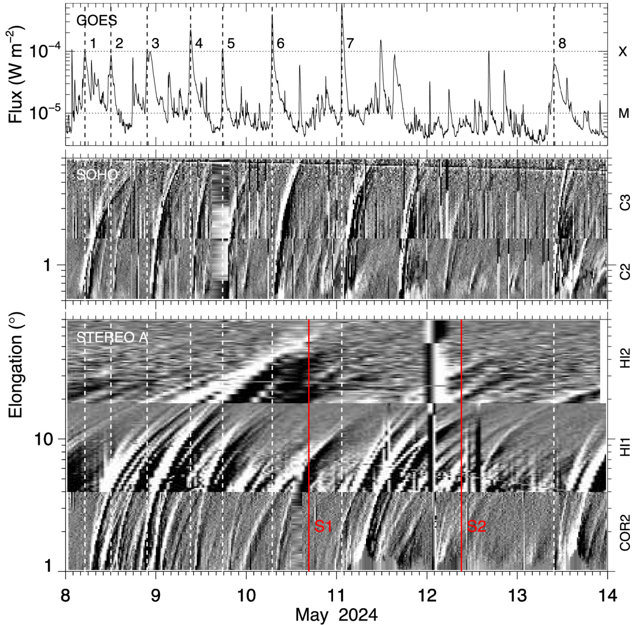
Figure 2. from Ying D. Liu et al 2024 Astrophys. J. Lett. 974 doi:10.3847/2041-8213/ad7ba4 https://dx.doi.org/10.3847/2041-8213/ad7ba4 © 2024. The Author(s). Published by the American Astronomical Society.
