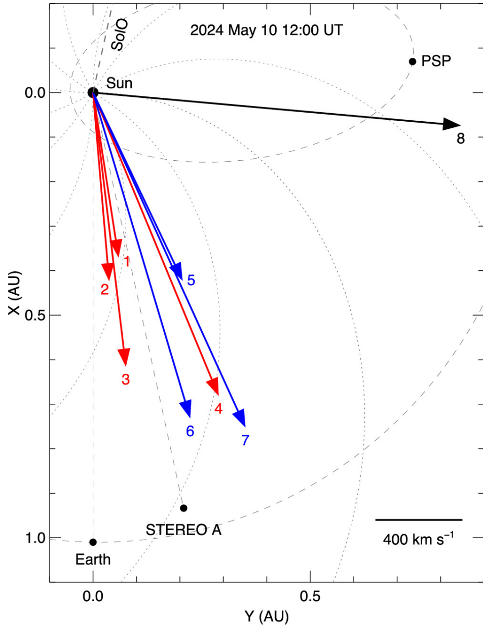
Figure 1. from Ying D. Liu et al 2024 Astrophys. J. Lett. 974 doi:10.3847/2041-8213/ad7ba4 https://dx.doi.org/10.3847/2041-8213/ad7ba4 © 2024. The Author(s). Published by the American Astronomical Society.
