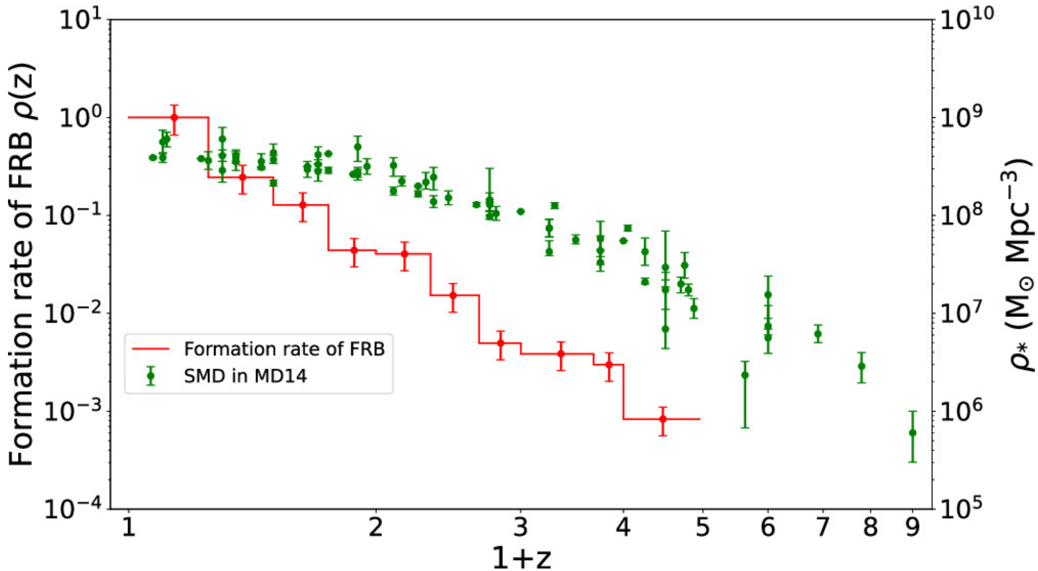
Figure 8. from J. H. Chen et al 2024 Astrophys. J. Lett. 973 doi:10.3847/2041-8213/ad7b39 https://dx.doi.org/10.3847/2041-8213/ad7b39 © 2024. The Author(s). Published by the American Astronomical Society.
