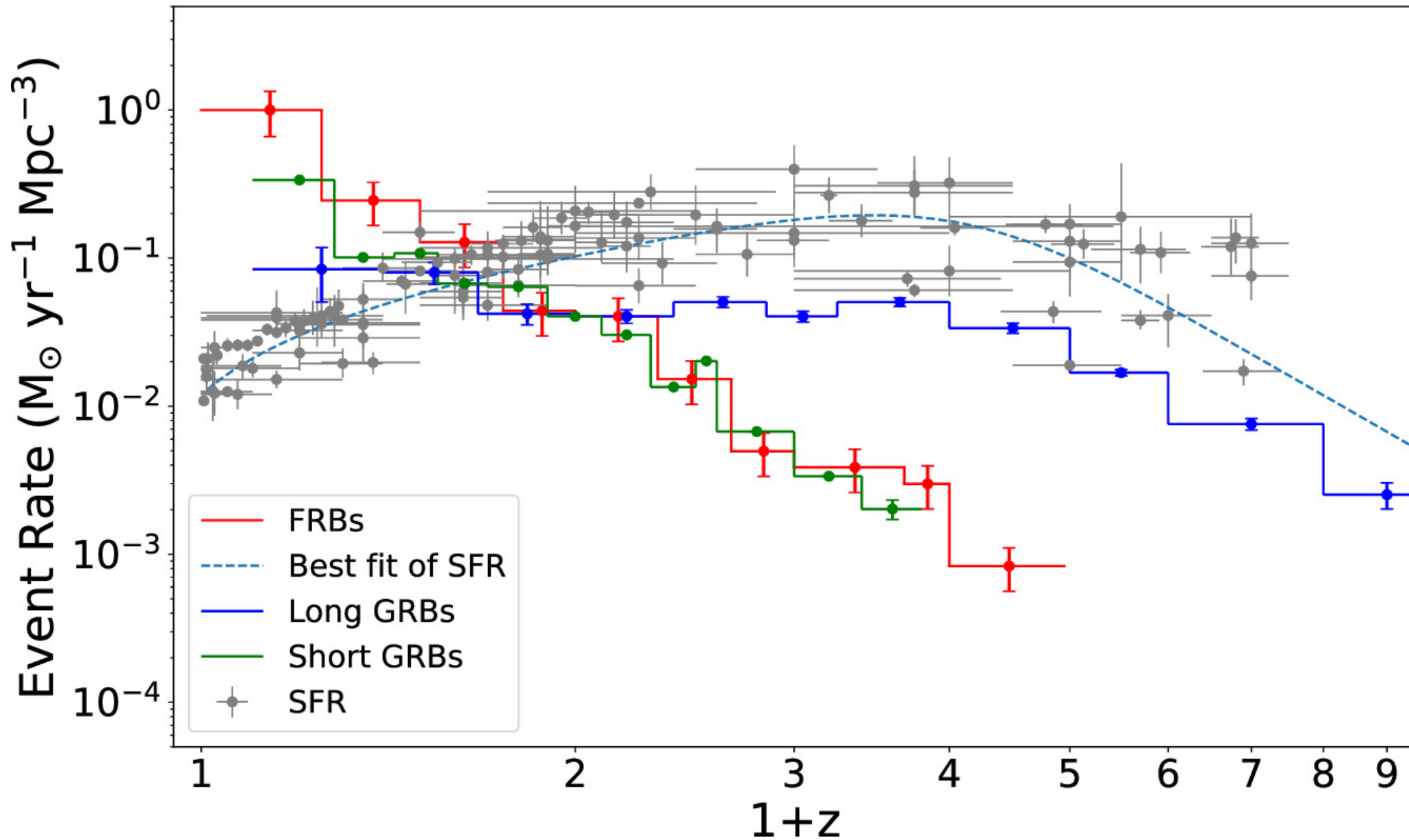
Figure 7. from J. H. Chen et al 2024 Astrophys. J. Lett. 973 doi:10.3847/2041-8213/ad7b39 https://dx.doi.org/10.3847/2041-8213/ad7b39 © 2024. The Author(s). Published by the American Astronomical Society.
