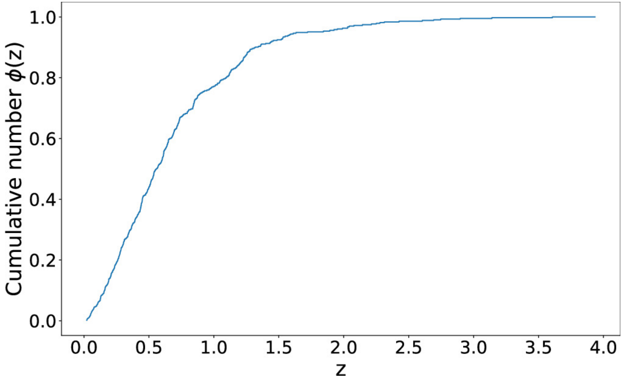
Figure 5. from J. H. Chen et al 2024 Astrophys. J. Lett. 973 doi:10.3847/2041-8213/ad7b39 https://dx.doi.org/10.3847/2041-8213/ad7b39 © 2024. The Author(s). Published by the American Astronomical Society.
