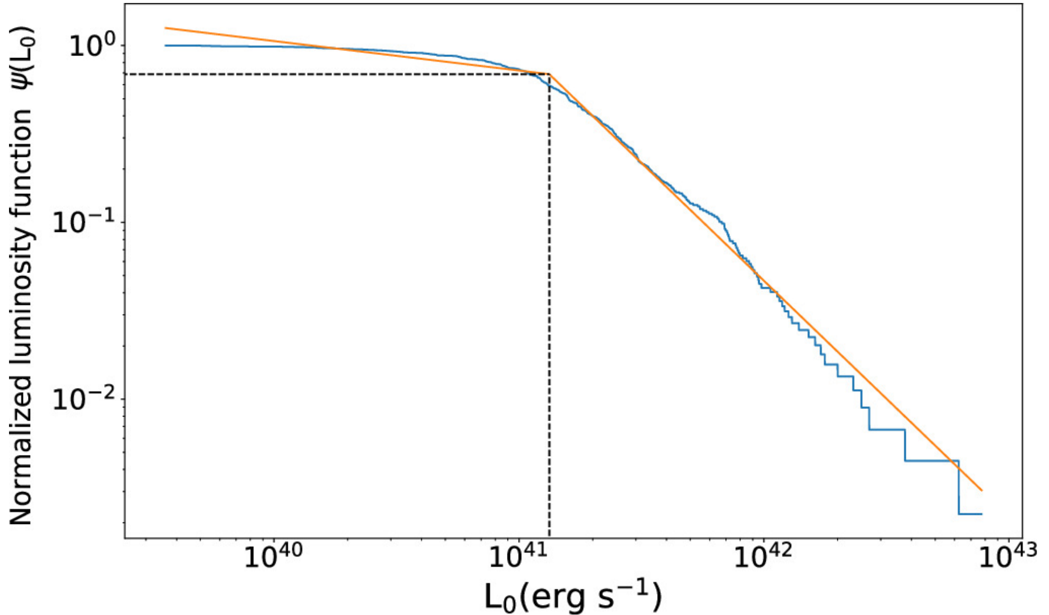
Figure 4. from J. H. Chen et al 2024 Astrophys. J. Lett. 973 doi:10.3847/2041-8213/ad7b39 https://dx.doi.org/10.3847/2041-8213/ad7b39 © 2024. The Author(s). Published by the American Astronomical Society.
