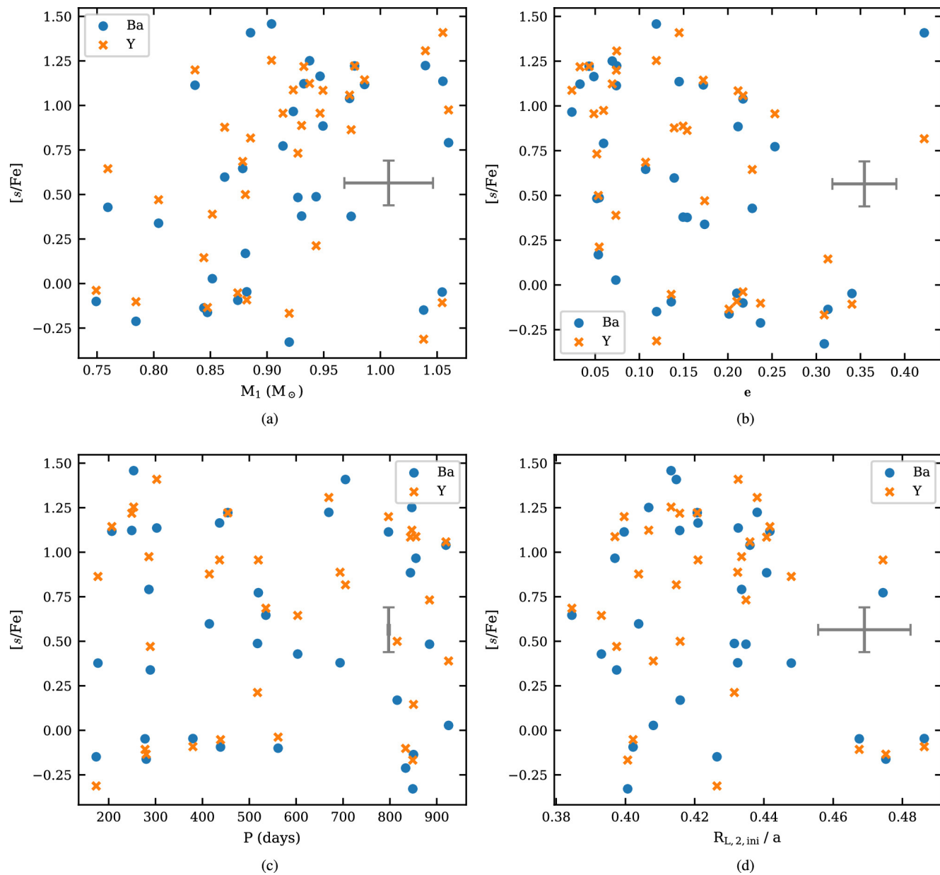
Figure 5. from Param Rekhi et al 2024 Astrophys. J. Lett. 973 doi:10.3847/2041-8213/ad77b9 https://dx.doi.org/10.3847/2041-8213/ad77b9 © 2024. The Author(s). Published by the American Astronomical Society.
