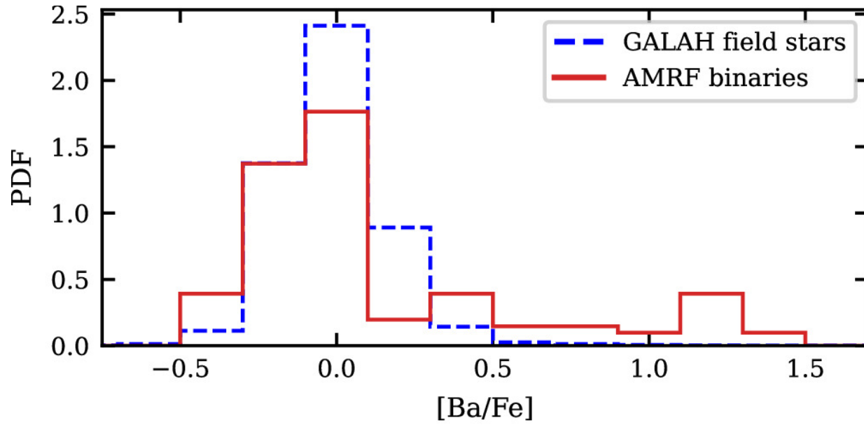
Figure 2. from Param Rekhi et al 2024 Astrophys. J. Lett. 973 doi:10.3847/2041-8213/ad77b9 https://dx.doi.org/10.3847/2041-8213/ad77b9 © 2024. The Author(s). Published by the American Astronomical Society.
