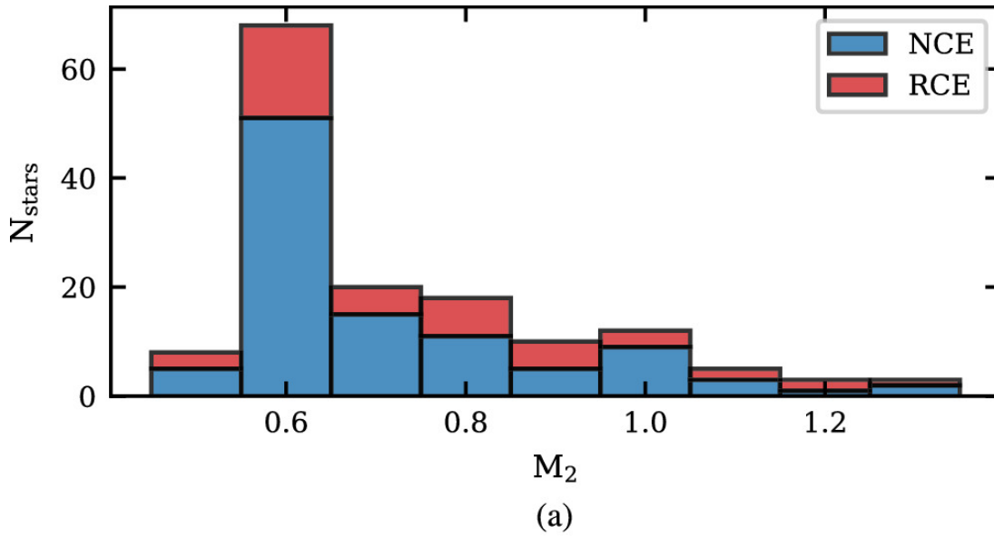
Figure 1. from Param Rekhi et al 2024 Astrophys. J. Lett. 973 doi:10.3847/2041-8213/ad77b9 https://dx.doi.org/10.3847/2041-8213/ad77b9 © 2024. The Author(s). Published by the American Astronomical Society.
