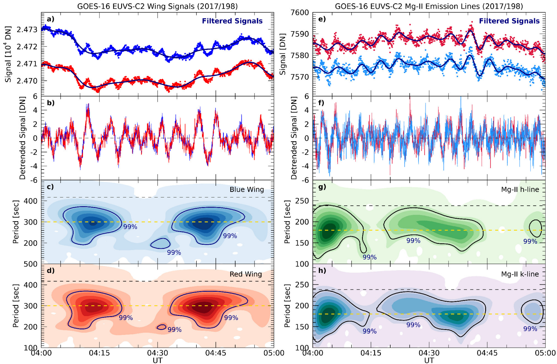
Figure 3. from Thomas D. Eden et al 2024 Astrophys. J. Lett. 973 doi:10.3847/2041-8213/ad73d9 https://dx.doi.org/10.3847/2041-8213/ad73d9 © 2024. The Author(s). Published by the American Astronomical Society.
