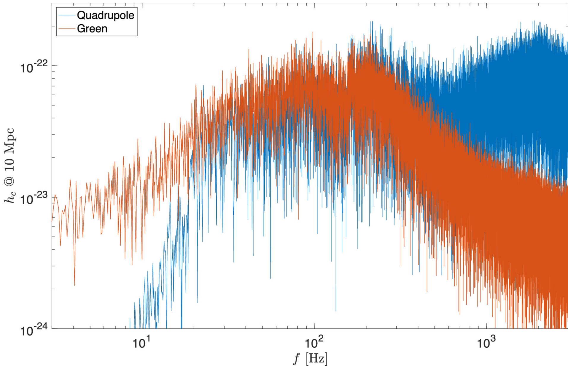
Figure 7. from Ore Gottlieb et al 2024 Astrophys. J. Lett. 972 doi:10.3847/2041-8213/ad697c https://dx.doi.org/10.3847/2041-8213/ad697c © 2024. The Author(s). Published by the American Astronomical Society.
