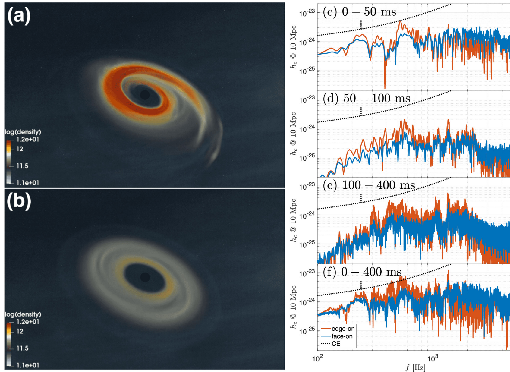
Figure 6. from Ore Gottlieb et al 2024 Astrophys. J. Lett. 972 doi:10.3847/2041-8213/ad697c https://dx.doi.org/10.3847/2041-8213/ad697c © 2024. The Author(s). Published by the American Astronomical Society.
