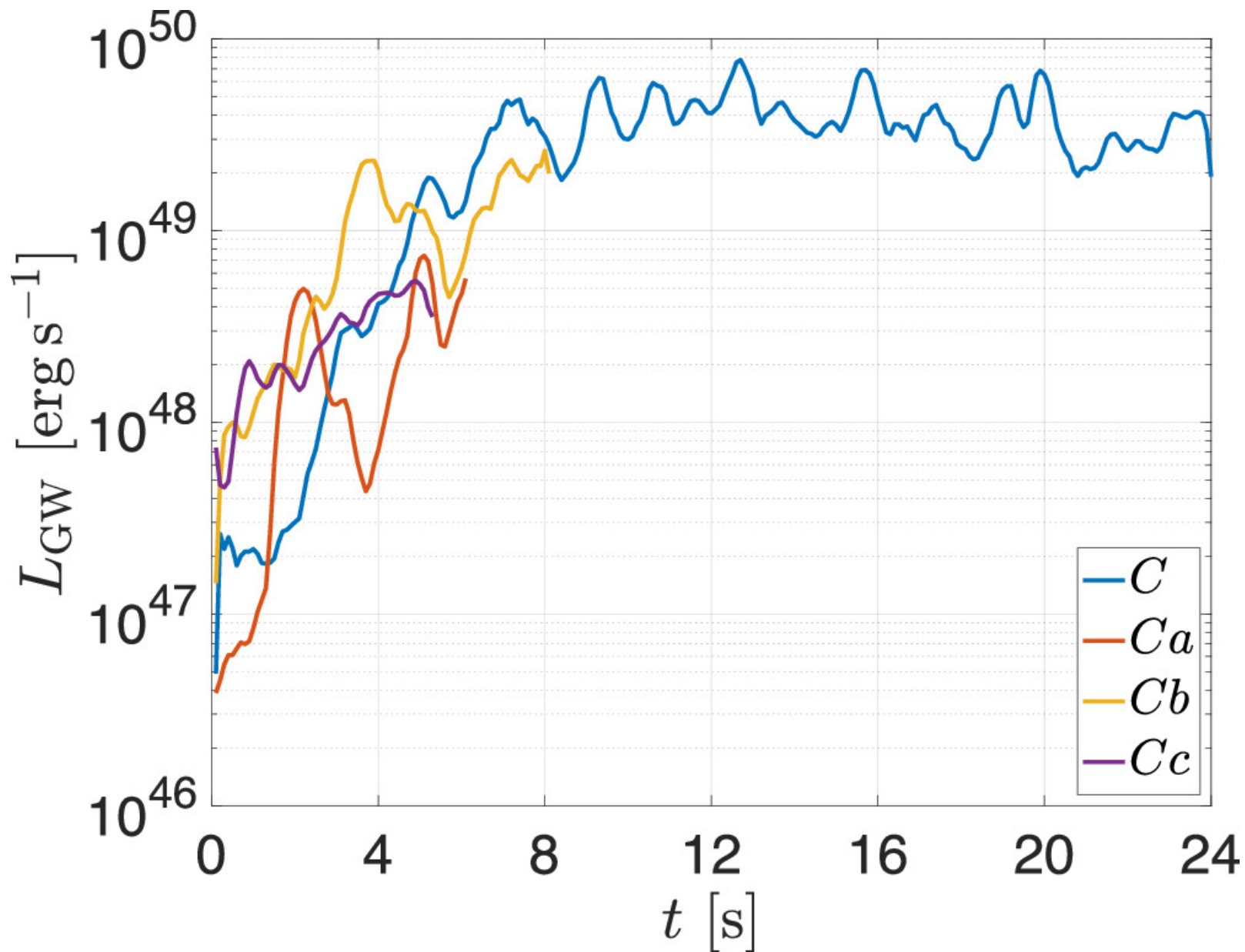
Figure 5. from Ore Gottlieb et al 2024 Astrophys. J. Lett. 972 doi:10.3847/2041-8213/ad697c https://dx.doi.org/10.3847/2041-8213/ad697c © 2024. The Author(s). Published by the American Astronomical Society.
