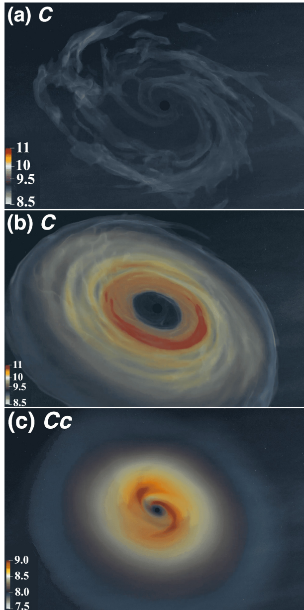
Figure 1. from Ore Gottlieb et al 2024 Astrophys. J. Lett. 972 doi:10.3847/2041-8213/ad697c https://dx.doi.org/10.3847/2041-8213/ad697c © 2024. The Author(s). Published by the American Astronomical Society.
