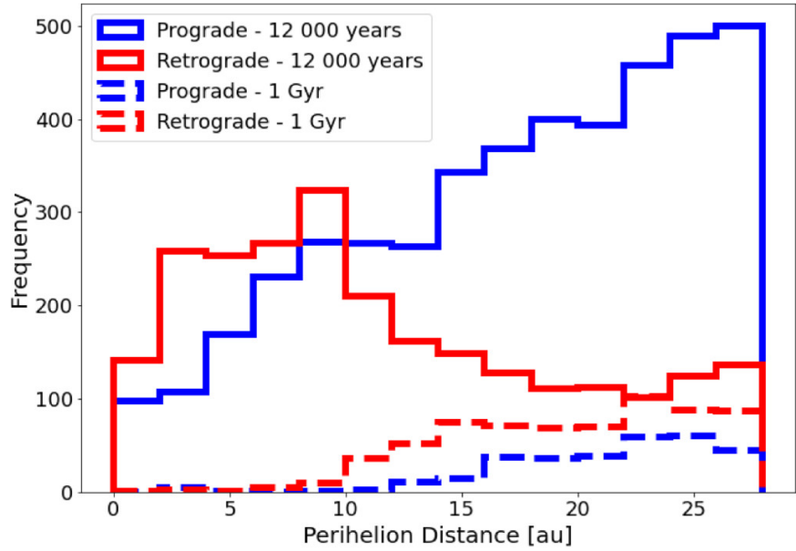
Figure 4. from Susanne Pfalzner et al 2024 Astrophys. J. Lett. 972 doi:10.3847/2041-8213/ad63a6 https://dx.doi.org/10.3847/2041-8213/ad63a6 © 2024. The Author(s). Published by the American Astronomical Society.
