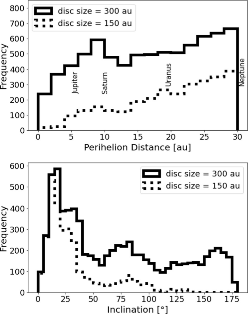
Figure 2. from Susanne Pfalzner et al 2024 Astrophys. J. Lett. 972 doi:10.3847/2041-8213/ad63a6 https://dx.doi.org/10.3847/2041-8213/ad63a6 © 2024. The Author(s). Published by the American Astronomical Society.
