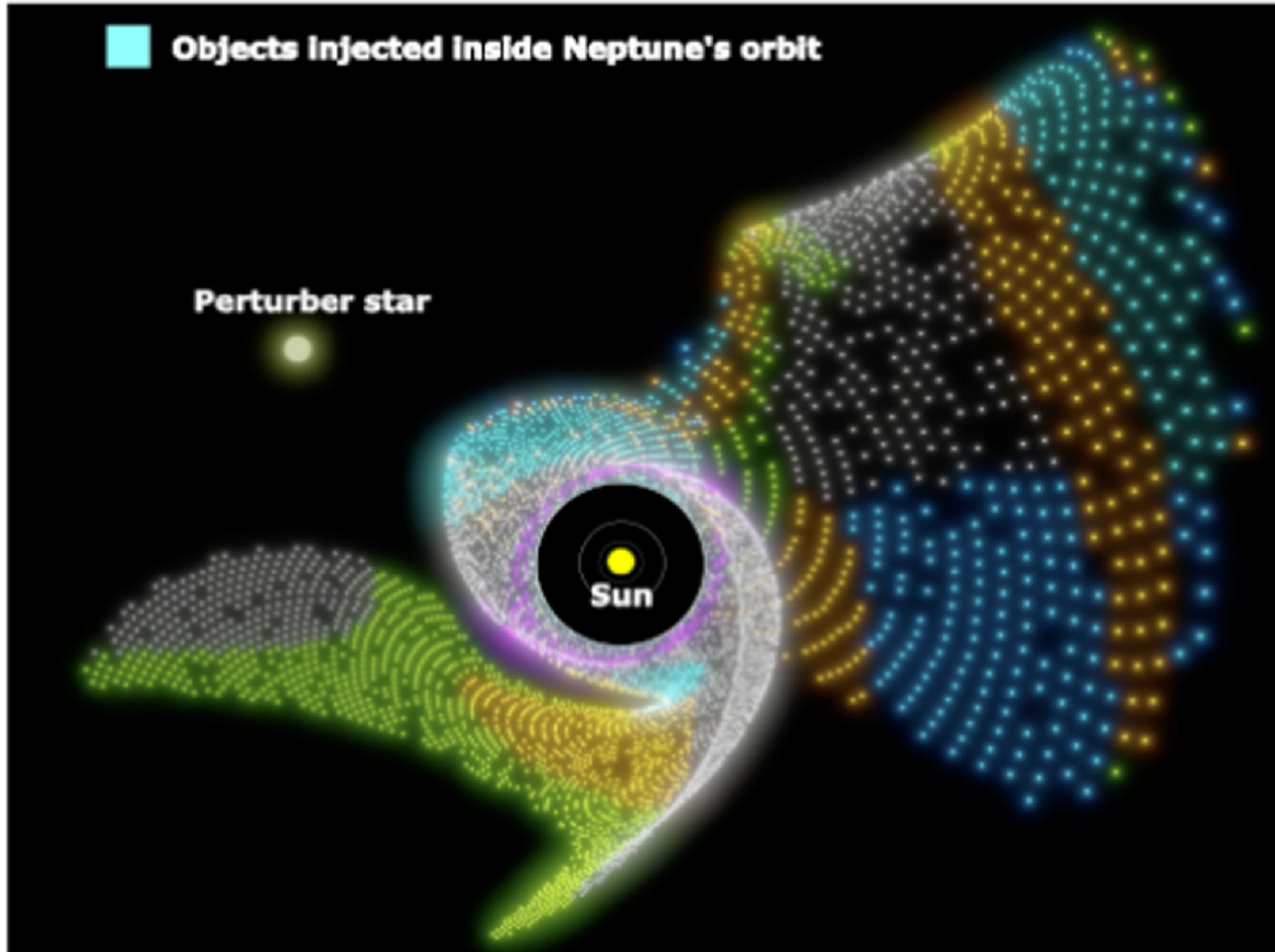
Figure 1. from Susanne Pfalzner et al 2024 Astrophys. J. Lett. 972 doi:10.3847/2041-8213/ad63a6 https://dx.doi.org/10.3847/2041-8213/ad63a6 © 2024. The Author(s). Published by the American Astronomical Society.
