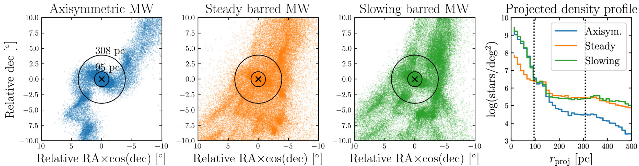
Figure 6. from Adam M. Dillamore et al 2024 Astrophys. J. Lett. 971 doi:10.3847/2041-8213/ad60c8 https://dx.doi.org/10.3847/2041-8213/ad60c8 © 2024. The Author(s). Published by the American Astronomical Society.
