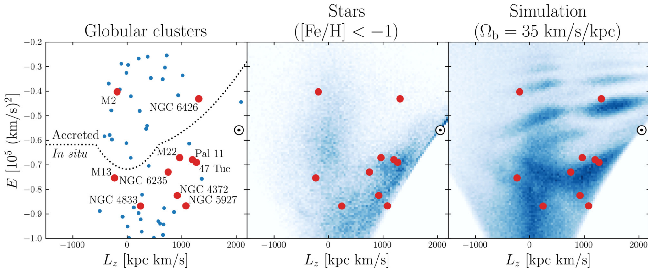
Figure 2. from Adam M. Dillamore et al 2024 Astrophys. J. Lett. 971 doi:10.3847/2041-8213/ad60c8 https://dx.doi.org/10.3847/2041-8213/ad60c8 © 2024. The Author(s). Published by the American Astronomical Society.
