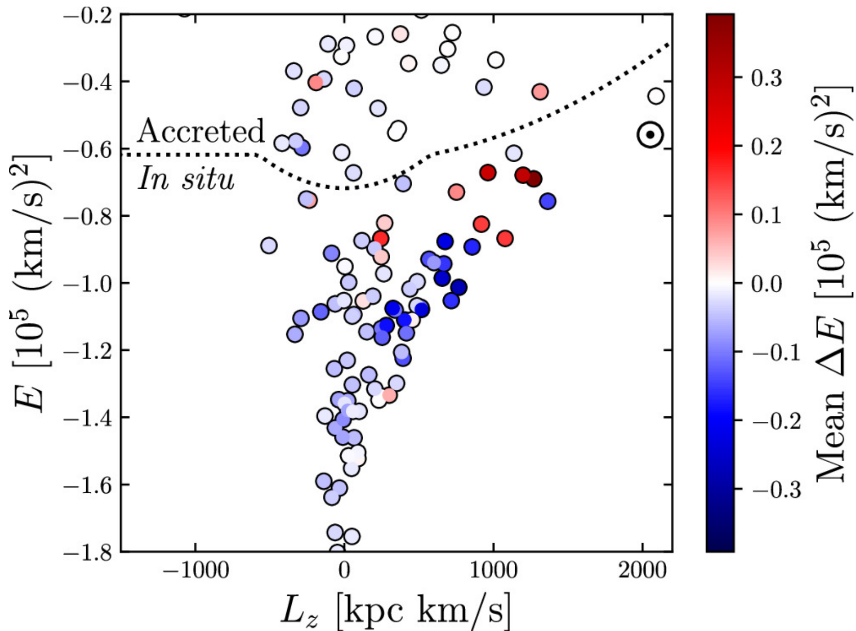
Figure 1. from Adam M. Dillamore et al 2024 Astrophys. J. Lett. 971 doi:10.3847/2041-8213/ad60c8 https://dx.doi.org/10.3847/2041-8213/ad60c8 © 2024. The Author(s). Published by the American Astronomical Society.
