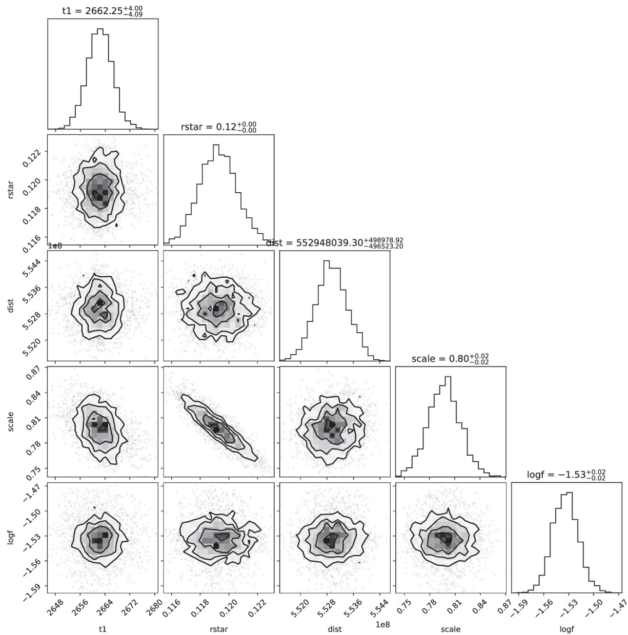
Figure 9. from Fatemeh Davoudi et al 2024 Astrophys. J. Lett. 970 doi:10.3847/2041-8213/ad5c6c https://dx.doi.org/10.3847/2041-8213/ad5c6c © 2024. The Author(s). Published by the American Astronomical Society.
