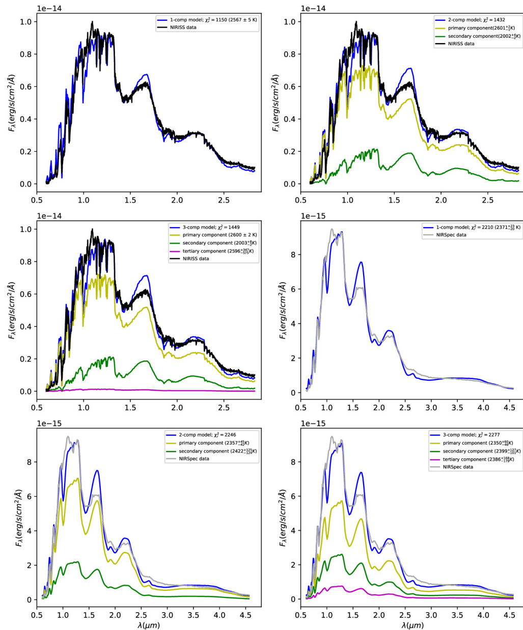
Figure 7. from Fatemeh Davoudi et al 2024 Astrophys. J. Lett. 970 doi:10.3847/2041-8213/ad5c6c https://dx.doi.org/10.3847/2041-8213/ad5c6c © 2024. The Author(s). Published by the American Astronomical Society.
