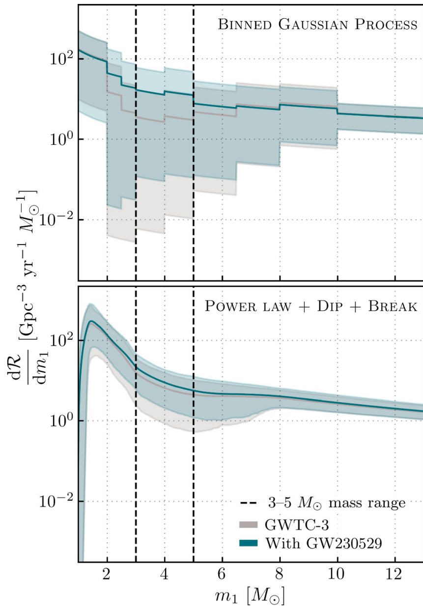
Figure 6. from A. G. Abac et al 2024 Astrophys. J. Lett. 970 doi:10.3847/2041-8213/ad5beb https://dx.doi.org/10.3847/2041-8213/ad5beb © 2024. The Author(s). Published by the American Astronomical Society.
