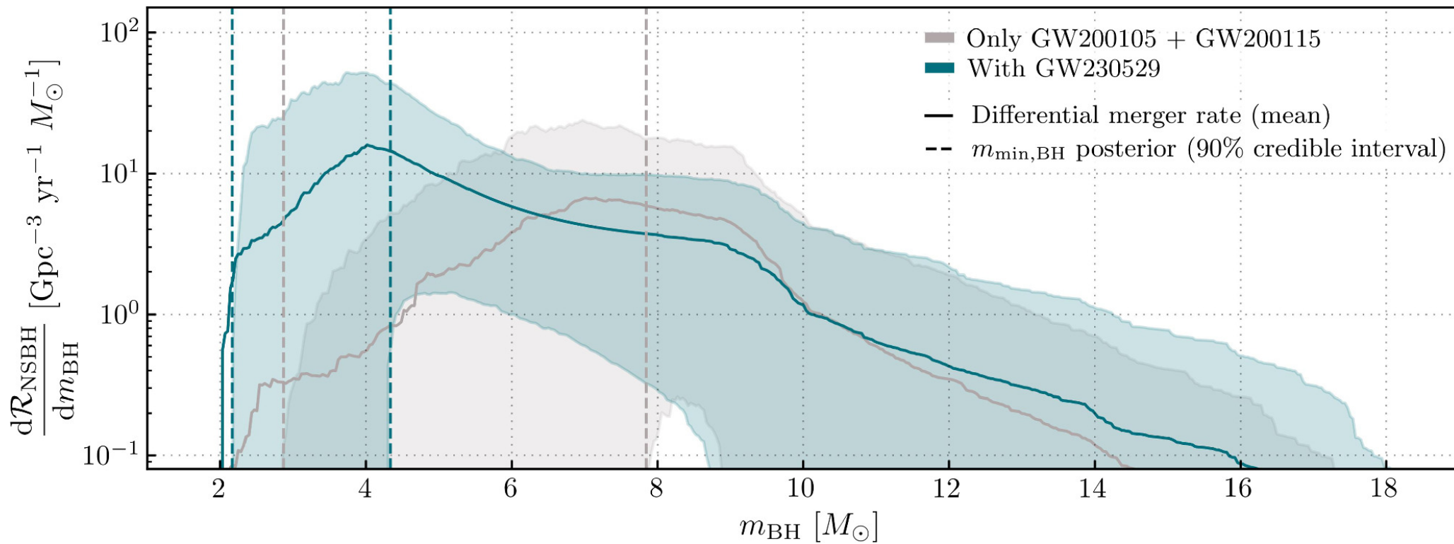
Figure 4. from A. G. Abac et al 2024 Astrophys. J. Lett. 970 doi:10.3847/2041-8213/ad5beb https://dx.doi.org/10.3847/2041-8213/ad5beb © 2024. The Author(s). Published by the American Astronomical Society.
