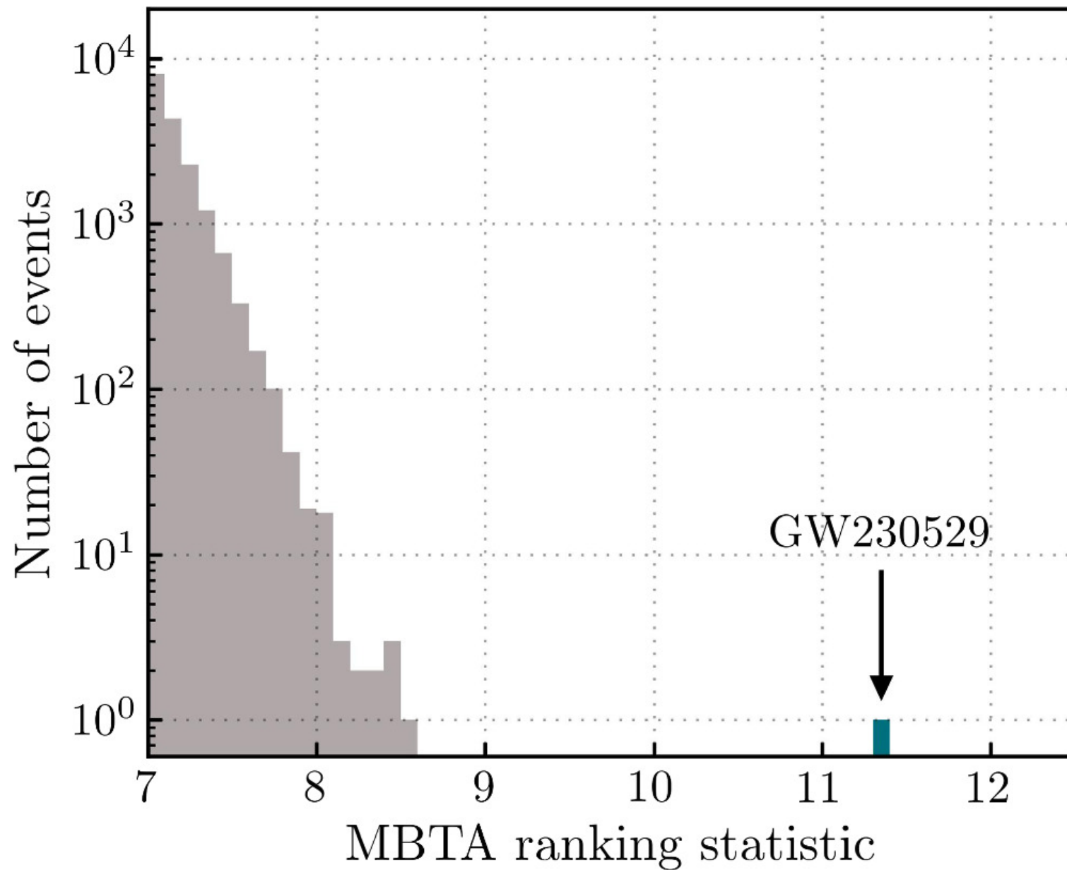
Figure 10. from A. G. Abac et al 2024 Astrophys. J. Lett. 970 doi:10.3847/2041-8213/ad5beb https://dx.doi.org/10.3847/2041-8213/ad5beb © 2024. The Author(s). Published by the American Astronomical Society.
