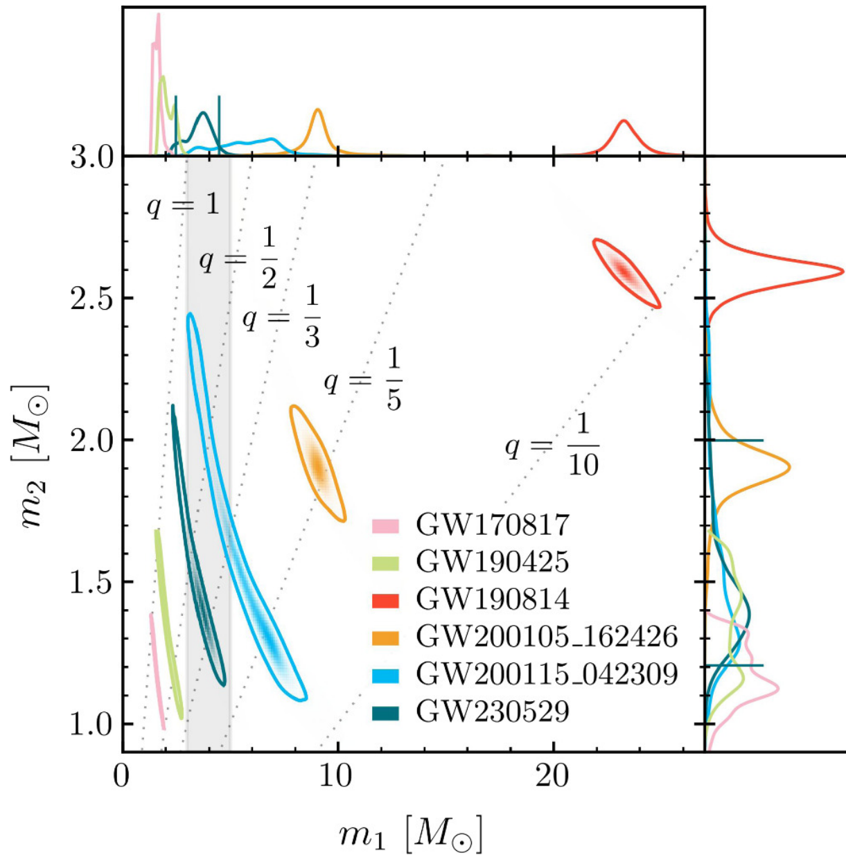
Figure 1. from A. G. Abac et al 2024 Astrophys. J. Lett. 970 doi:10.3847/2041-8213/ad5beb https://dx.doi.org/10.3847/2041-8213/ad5beb © 2024. The Author(s). Published by the American Astronomical Society.
