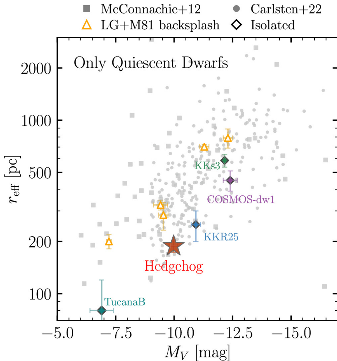
Figure 4. from Jiaxuan Li et al 2024 Astrophys. J. Lett. 975 doi:10.3847/2041-8213/ad5b59 https://dx.doi.org/10.3847/2041-8213/ad5b59 © 2024. The Author(s). Published by the American Astronomical Society.
