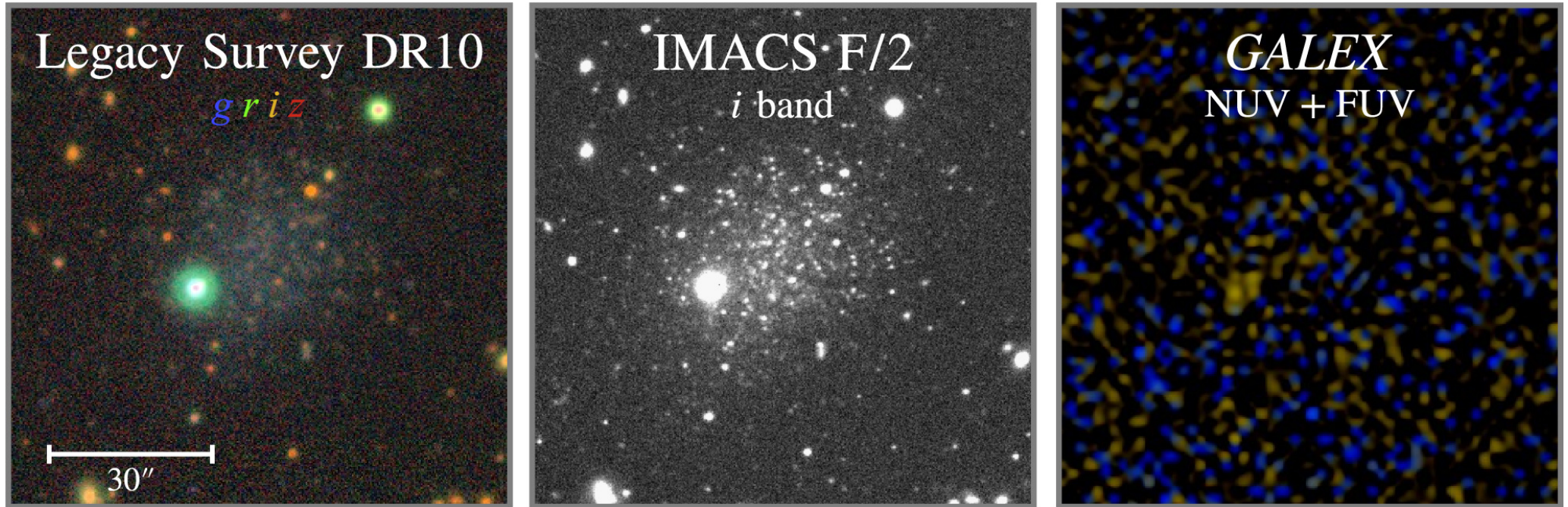
Figure 1. from Jiaxuan Li et al 2024 Astrophys. J. Lett. 975 doi:10.3847/2041-8213/ad5b59 https://dx.doi.org/10.3847/2041-8213/ad5b59 © 2024. The Author(s). Published by the American Astronomical Society.
