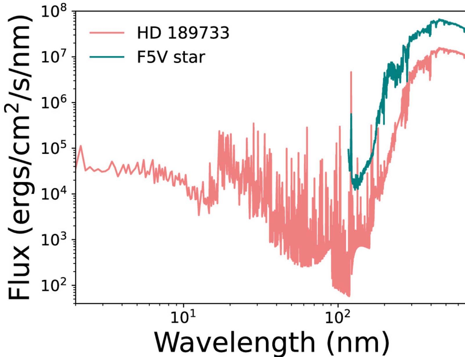
Figure 3. from Arjun B. Savel et al 2024 Astrophys. J. Lett. 969 doi:10.3847/2041-8213/ad5a0a https://dx.doi.org/10.3847/2041-8213/ad5a0a © 2024. The Author(s). Published by the American Astronomical Society.
