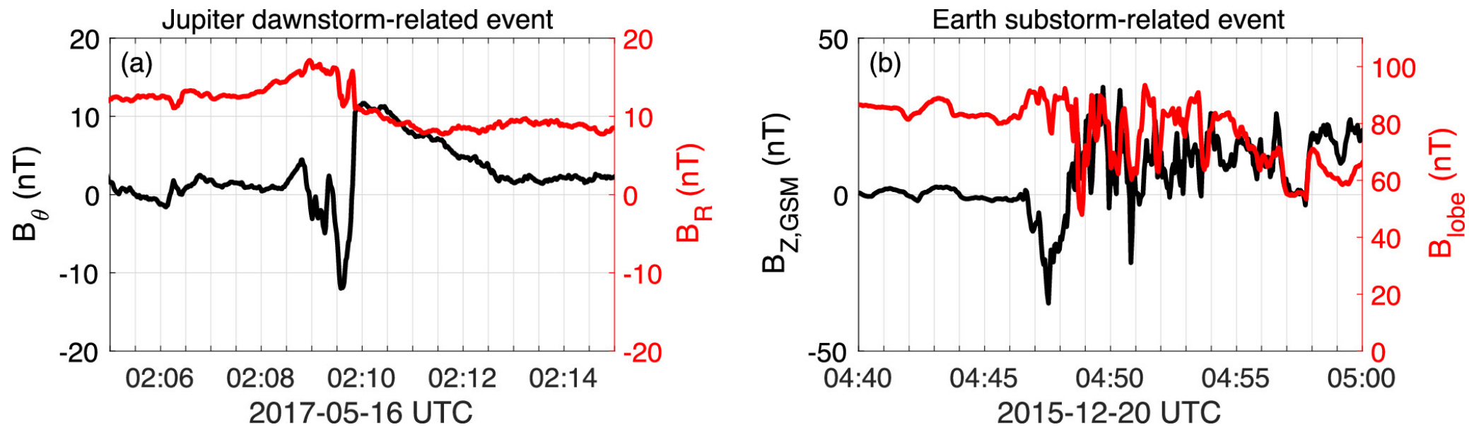
Figure 3. from Dong-Xiao Pan et al 2024 Astrophys. J. Lett. 969 doi:10.3847/2041-8213/ad5962 https://dx.doi.org/10.3847/2041-8213/ad5962 © 2024. The Author(s). Published by the American Astronomical Society.
