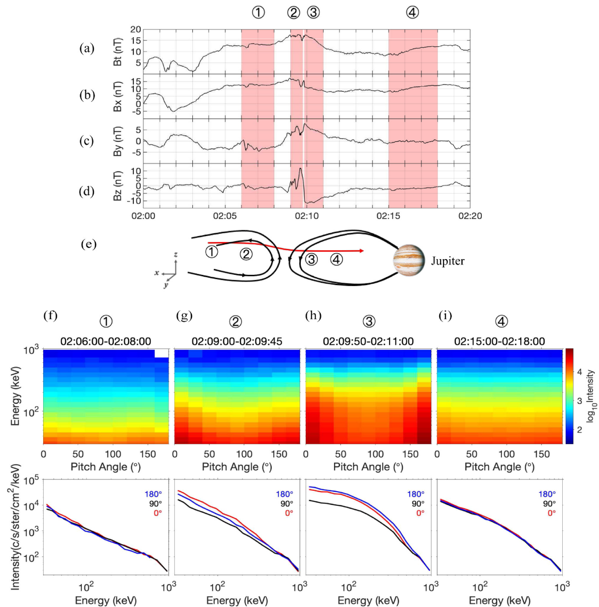
Figure 2. from Dong-Xiao Pan et al 2024 Astrophys. J. Lett. 969 doi:10.3847/2041-8213/ad5962 https://dx.doi.org/10.3847/2041-8213/ad5962 © 2024. The Author(s). Published by the American Astronomical Society.
