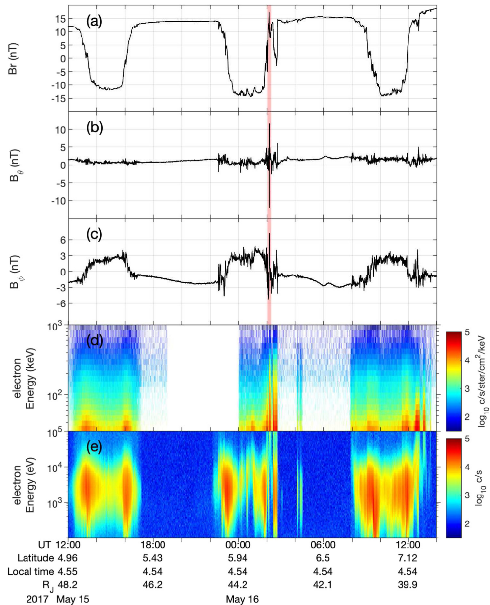
Figure 1. from Dong-Xiao Pan et al 2024 Astrophys. J. Lett. 969 doi:10.3847/2041-8213/ad5962 https://dx.doi.org/10.3847/2041-8213/ad5962 © 2024. The Author(s). Published by the American Astronomical Society.
