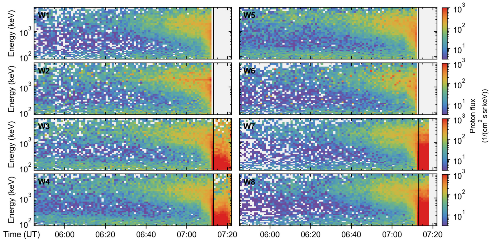
Figure 8. from Immanuel Christopher Jebaraj et al 2024 Astrophys. J. Lett. 968 doi:10.3847/2041-8213/ad4daa https://dx.doi.org/10.3847/2041-8213/ad4daa © 2024. The Author(s). Published by the American Astronomical Society.
