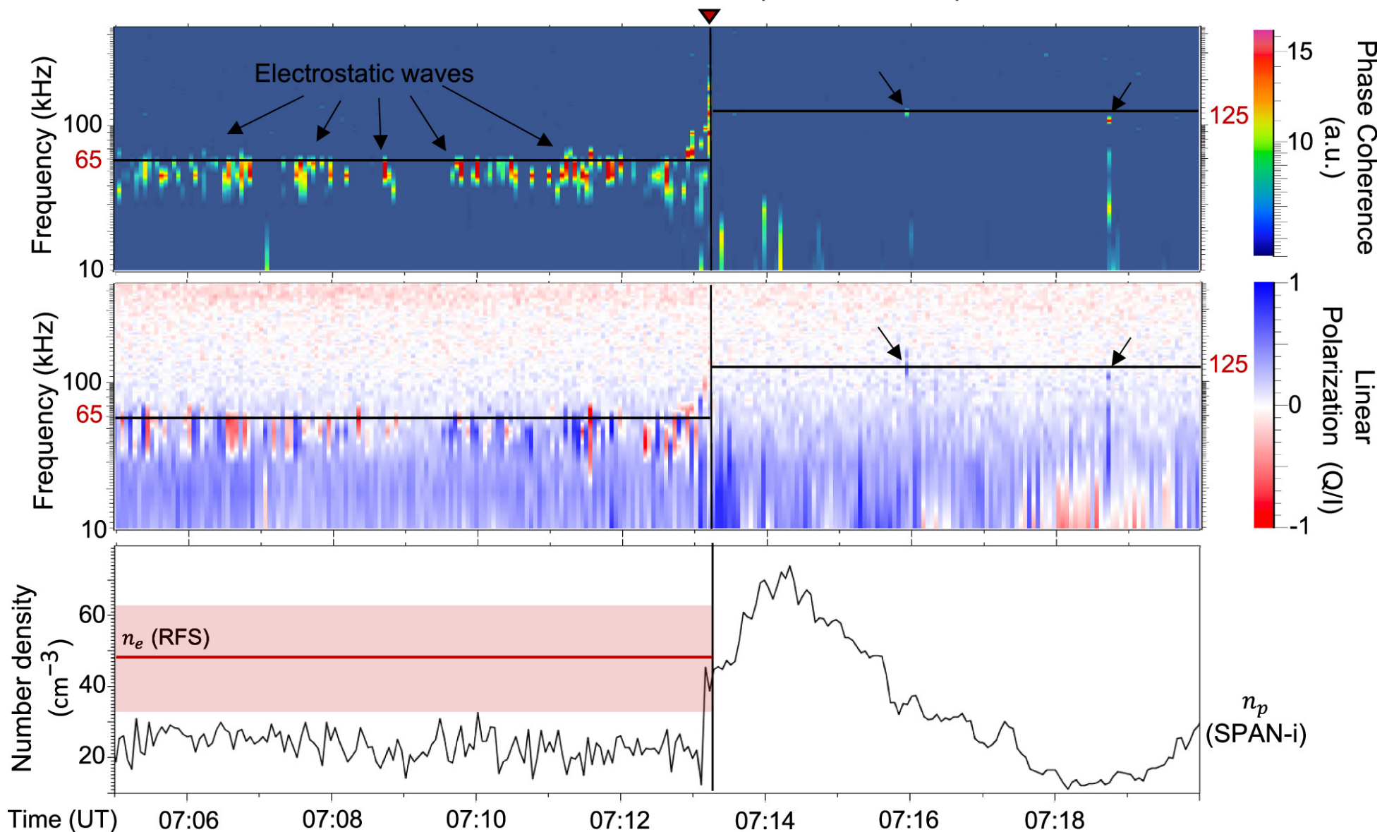
Figure 5. from Immanuel Christopher Jebaraj et al 2024 Astrophys. J. Lett. 968 doi:10.3847/2041-8213/ad4daa https://dx.doi.org/10.3847/2041-8213/ad4daa © 2024. The Author(s). Published by the American Astronomical Society.
