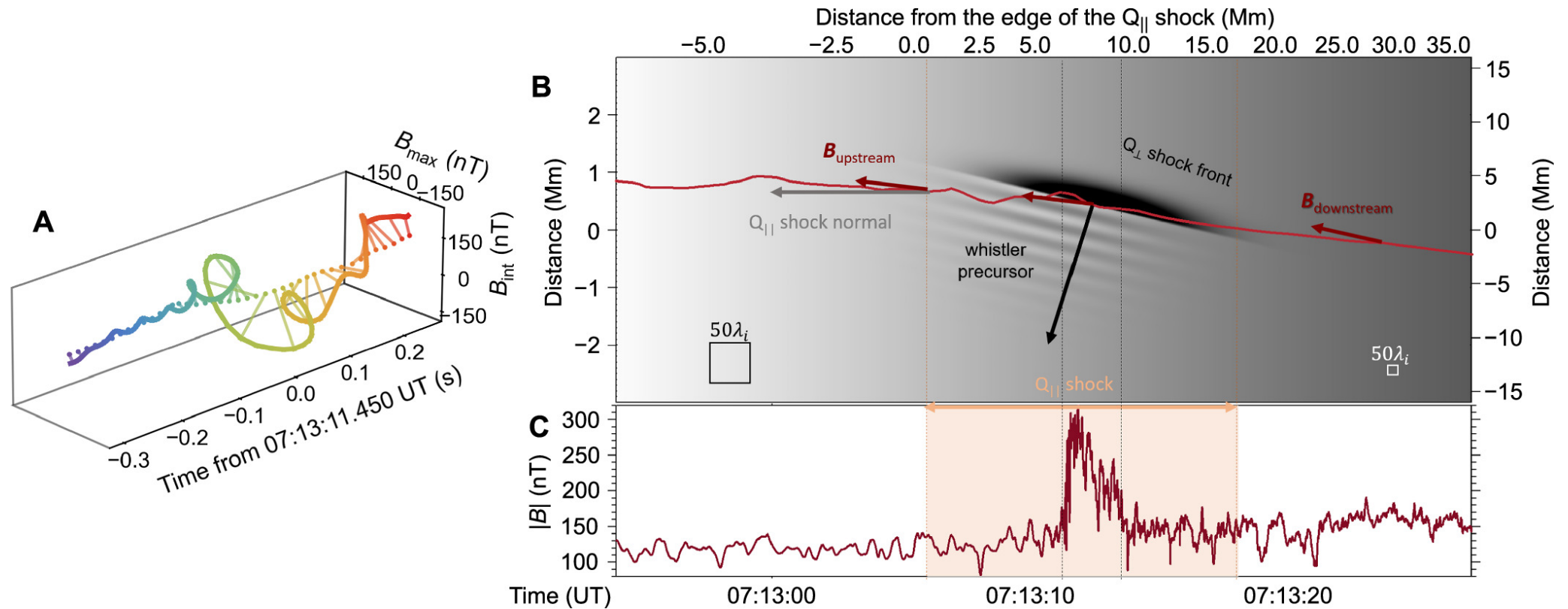
Figure 4. from Immanuel Christopher Jebaraj et al 2024 Astrophys. J. Lett. 968 doi:10.3847/2041-8213/ad4daa https://dx.doi.org/10.3847/2041-8213/ad4daa © 2024. The Author(s). Published by the American Astronomical Society.
