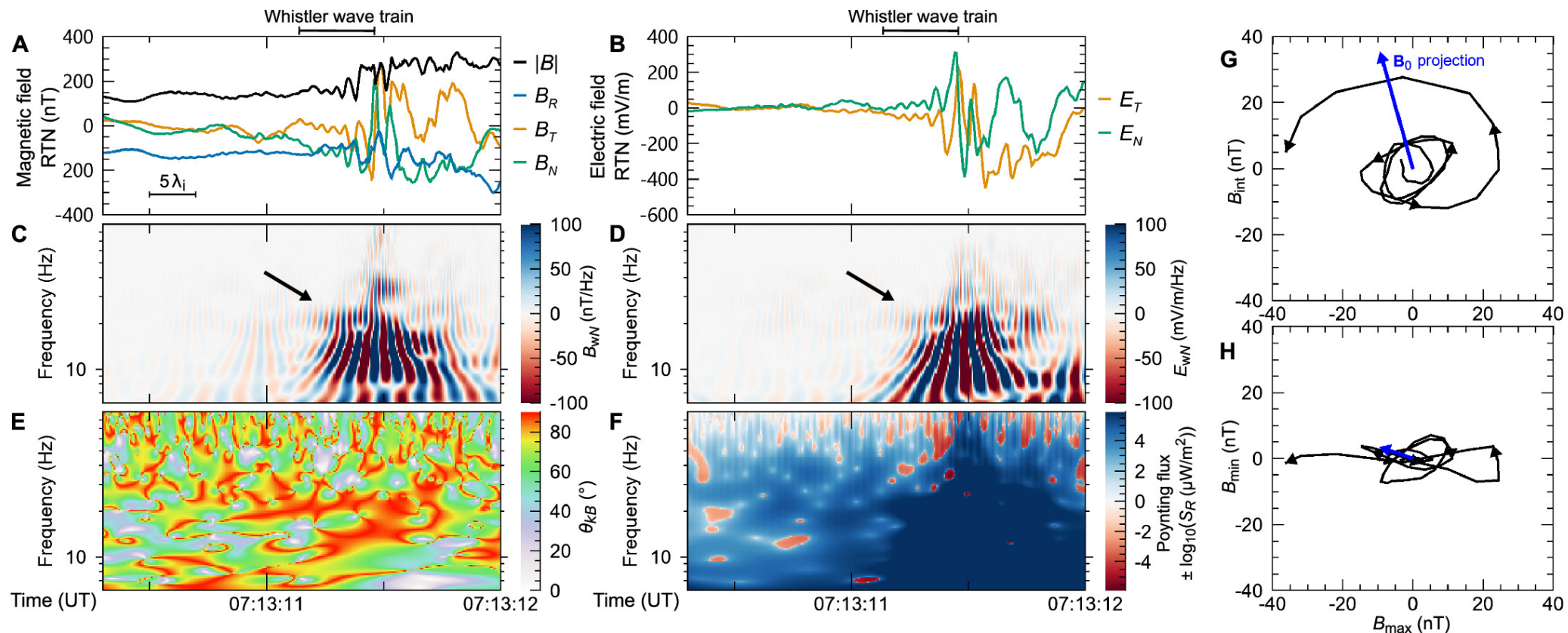
Figure 3. from Immanuel Christopher Jebaraj et al 2024 Astrophys. J. Lett. 968 doi:10.3847/2041-8213/ad4daa https://dx.doi.org/10.3847/2041-8213/ad4daa © 2024. The Author(s). Published by the American Astronomical Society.
