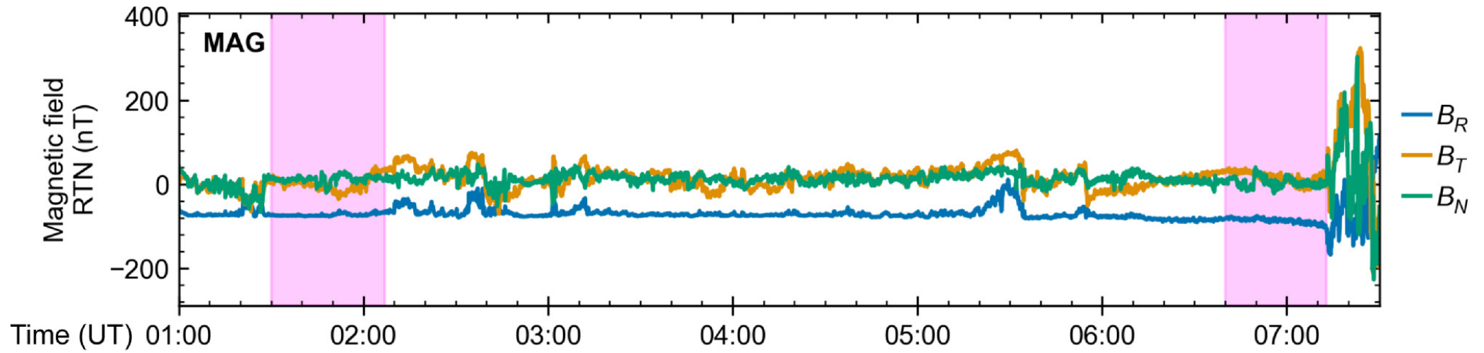
Figure 10. from Immanuel Christopher Jebaraj et al 2024 Astrophys. J. Lett. 968 doi:10.3847/2041-8213/ad4daa https://dx.doi.org/10.3847/2041-8213/ad4daa © 2024. The Author(s). Published by the American Astronomical Society.
