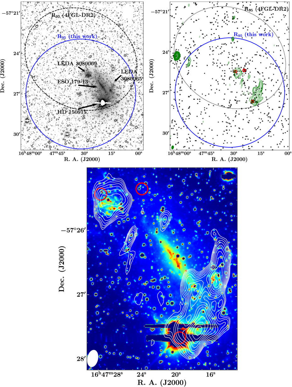
Figure 1. from Vaidehi S. Paliya and D. J. Saikia 2024 Astrophys. J. Lett. 967 doi:10.3847/2041-8213/ad4999 https://dx.doi.org/10.3847/2041-8213/ad4999 © 2024. The Author(s). Published by the American Astronomical Society.
