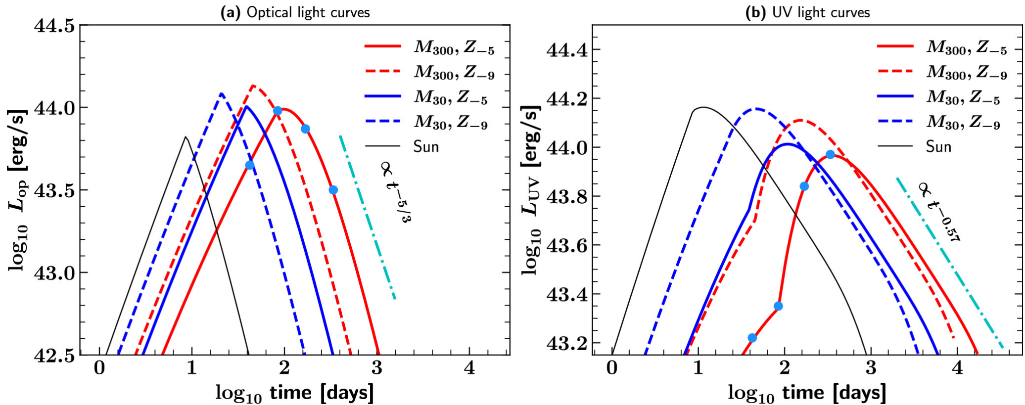
Figure 7. from Rudrani Kar Chowdhury et al 2024 Astrophys. J. Lett. 966 doi:10.3847/2041-8213/ad41b7 https://dx.doi.org/10.3847/2041-8213/ad41b7 © 2024. The Author(s). Published by the American Astronomical Society.
