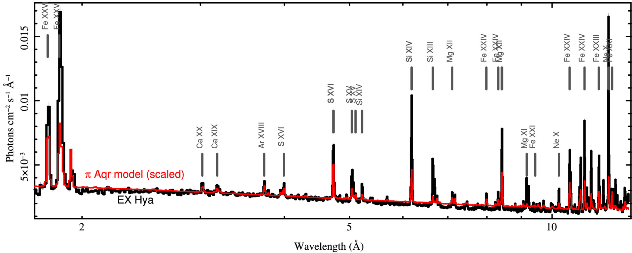
Figure 3. from David P. Huenemoerder et al 2024 Astrophys. J. Lett. 966 doi:10.3847/2041-8213/ad4095 https://dx.doi.org/10.3847/2041-8213/ad4095 © 2024. The Author(s). Published by the American Astronomical Society.
