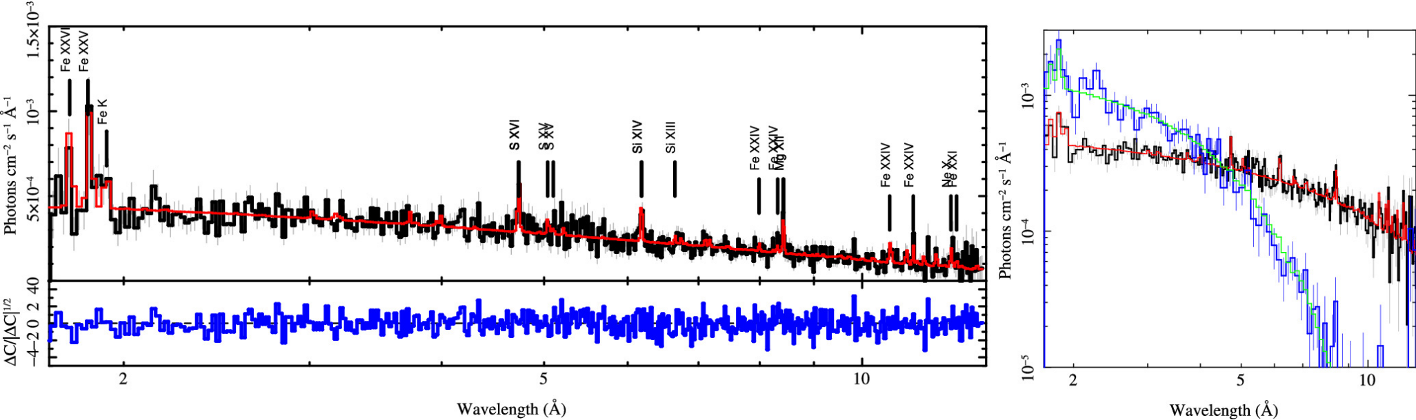
Figure 1. from David P. Huenemoerder et al 2024 Astrophys. J. Lett. 966 doi:10.3847/2041-8213/ad4095 https://dx.doi.org/10.3847/2041-8213/ad4095 © 2024. The Author(s). Published by the American Astronomical Society.
