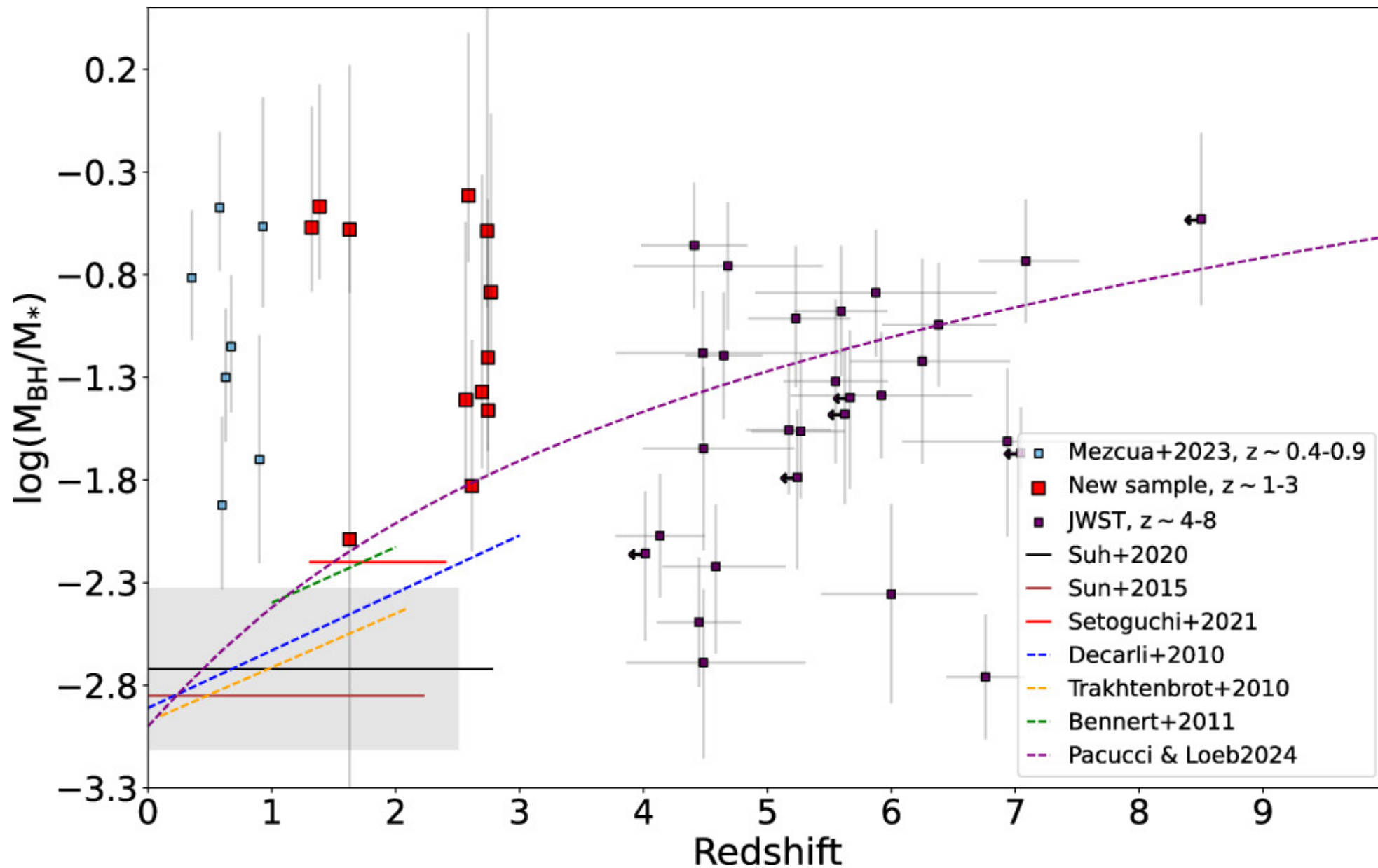
Figure 2. from Mar Mezcu et al 2024 Astrophys. J. Lett. 966 doi:10.3847/2041-8213/ad3c2a https://dx.doi.org/10.3847/2041-8213/ad3c2a © 2024. The Author(s). Published by the American Astronomical Society.
