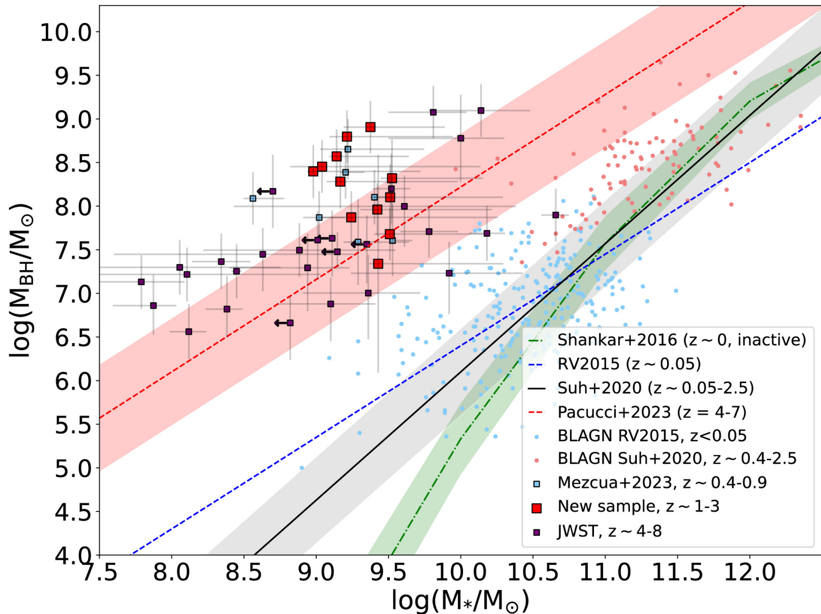
Figure 1. from Mar Mezcuca et al 2024 Astrophys. J. Lett. 966 doi:10.3847/2041-8213/ad3c2a https://dx.doi.org/10.3847/2041-8213/ad3c2a © 2024. The Author(s). Published by the American Astronomical Society.
