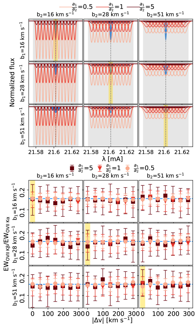
Figure 4. from Sanskriti Das 2024 Astrophys. J. Lett. 963 doi:10.3847/2041-8213/ad2a43 https://dx.doi.org/10.3847/2041-8213/ad2a43 © 2024. The Author(s). Published by the American Astronomical Society.
