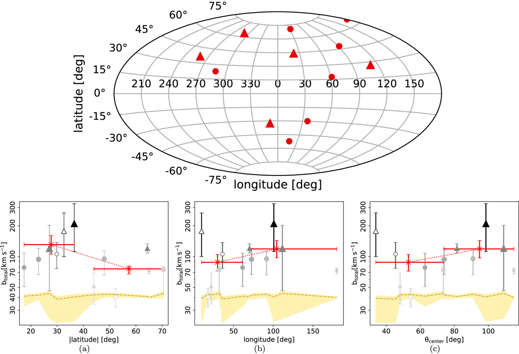
Figure 3. from Sanskriti Das 2024 Astrophys. J. Lett. 963 doi:10.3847/2041-8213/ad2a43 https://dx.doi.org/10.3847/2041-8213/ad2a43 © 2024. The Author(s). Published by the American Astronomical Society.
