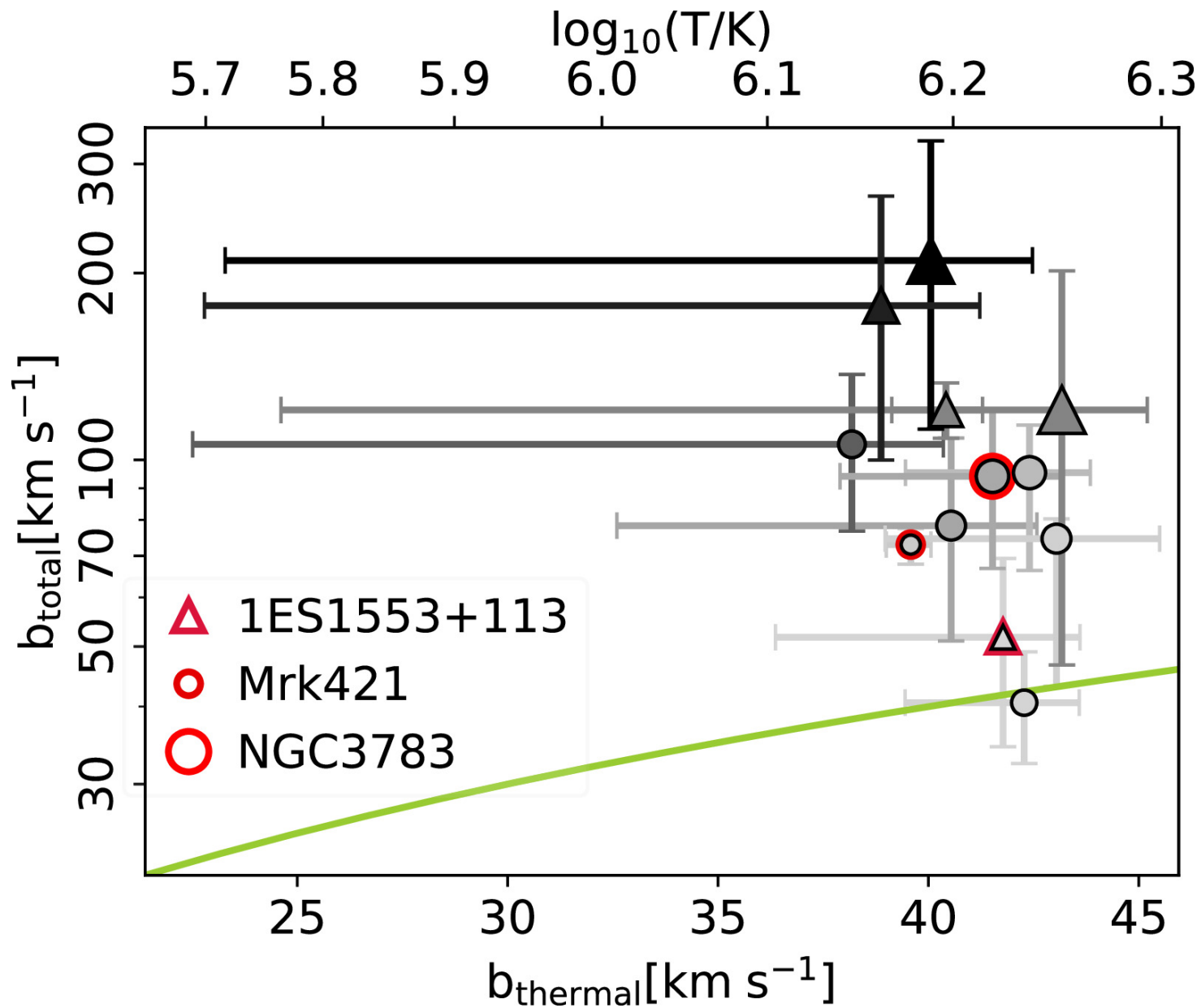
Figure 2. from Sanskriti Das 2024 Astrophys. J. Lett. 963 doi:10.3847/2041-8213/ad2a43 https://dx.doi.org/10.3847/2041-8213/ad2a43 © 2024. The Author(s). Published by the American Astronomical Society.
